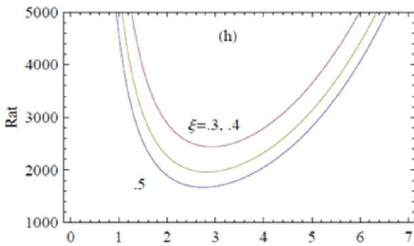
Fig. 2: Variation of Oscillatory Rayleigh number with wave number for the different values of \xi
