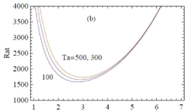
Fig.1: Variation of Stationary Rayleigh number with wave number for the different values of T_a
