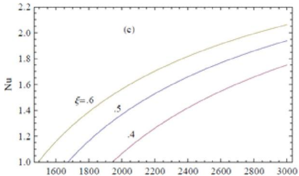
Fig.3: Variation of Nusselt number with Rayleigh number for the different values of \xi
