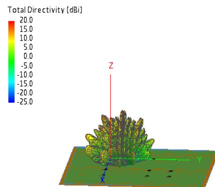
Figure 4: Total directivity in dB
