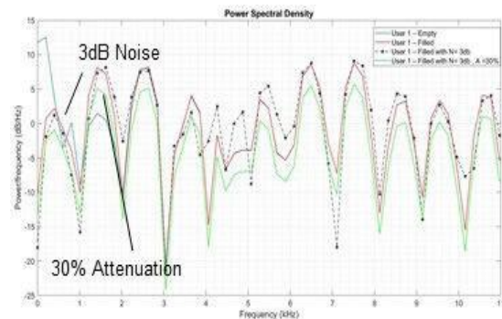
Figure 12: Frequency noise and attenuation
