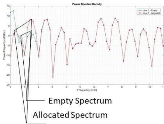
Figure 9: Frequency comparison when and not allocated
