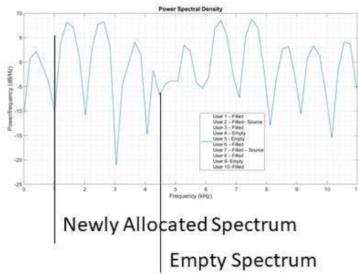
Figure 8: One new user added and one empty space
